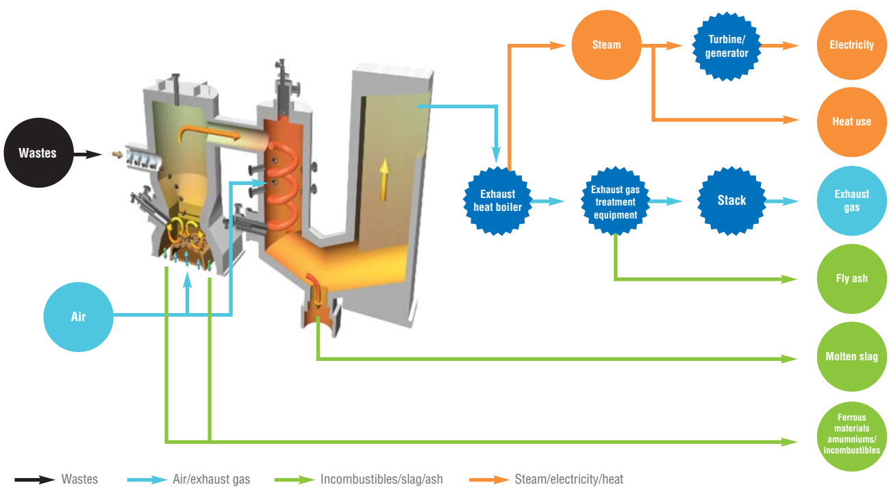
Fluidized-bed gasification and ash melting system TIGF
